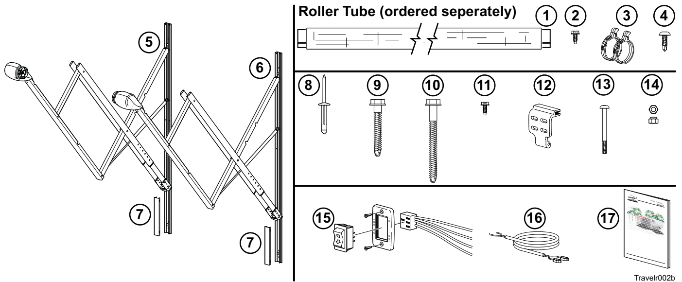
Figure 2. Component Checklist.
