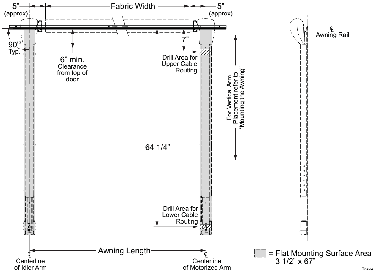
Figure 1. General Layout.
