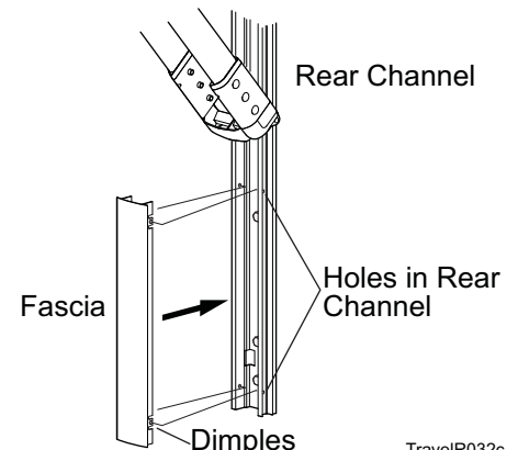
Figure 14. Attaching the Fascia.
