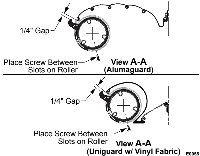
Figure 13. Installing the Tractioner.
